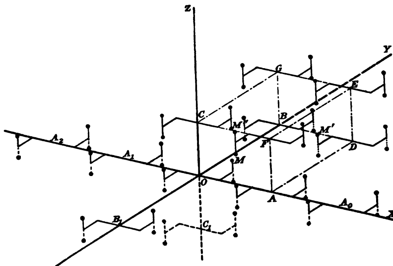
FIG. 20. A portion from the monoclinic space-group C_{2h}^1 .
